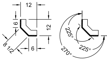
DR686270 6"x8 1/2"x6"x270° Double Reverse
